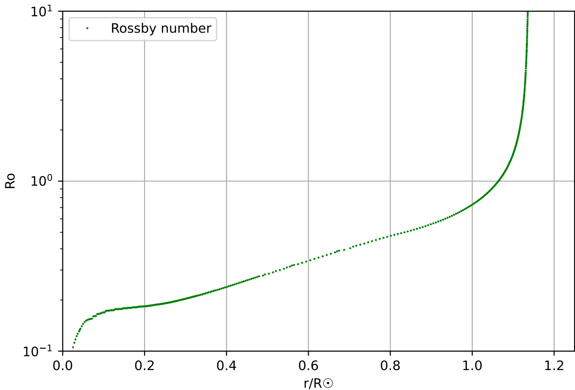
Rossby number, profile 163, age 8.14 \times 10^9
